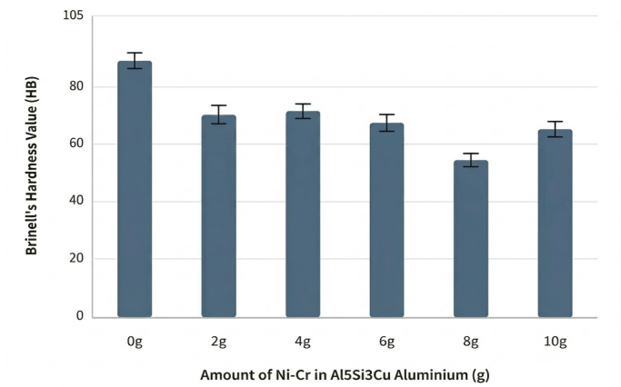
Figure 6. Brinell hardness values (HB) of Al5Si3Cu aluminium alloy reinforced with Ni-Cr (0–10 g). Error bars represent ± one standard deviation from triplicate measurements ( n = 3 ).
