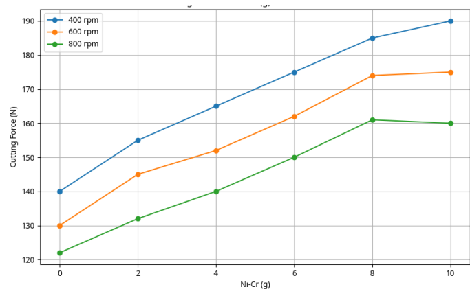
Figure 10. Cutting force vs. percentage of Ni-Cr in Al5Si3Cu.
