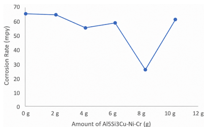
Figure 15. Corrosion level of reinforced Al5Si3Cu-Ni-Cr.
