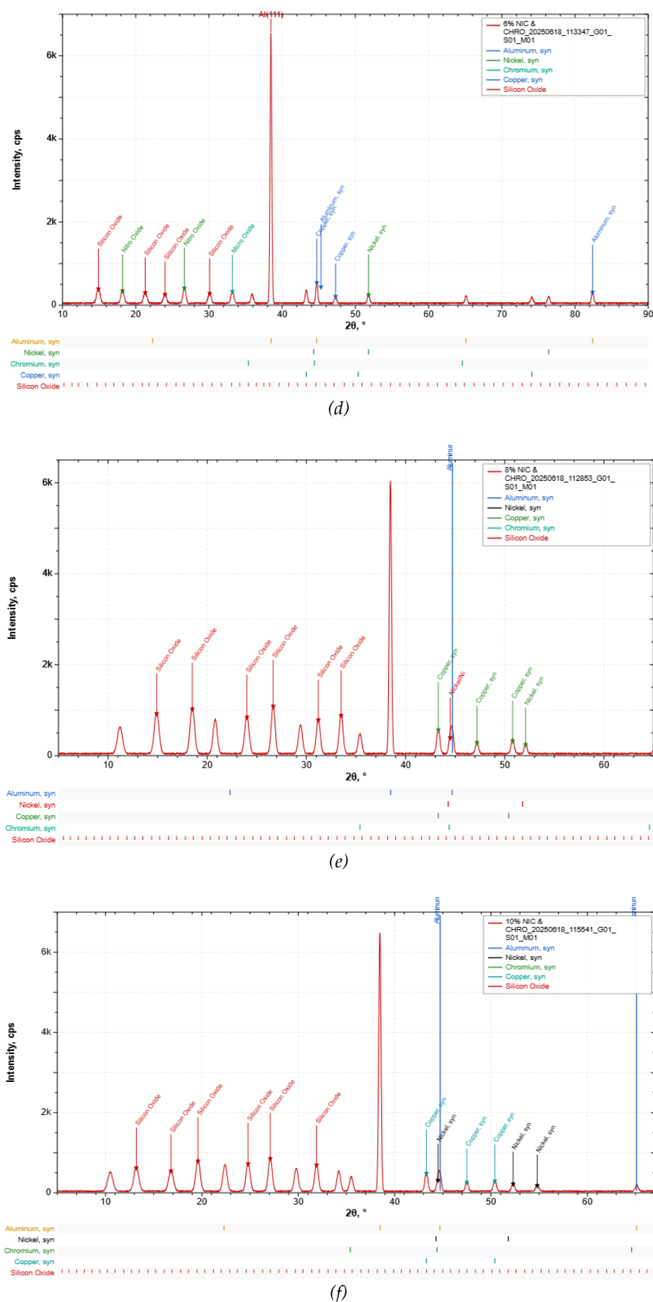
Figure 12. (a) Pure Al5Si3Cu (b) reinforced Al5Si3Cu with 2g of Ni-Cr (c) reinforced Al5Si3Cu with 4g of Ni-Cr, (d) reinforced Al5Si3Cu with 6g of Ni-Cr (e) reinforced Al5Si3Cu with 8g of Ni-Cr and (f) reinforced Al5Si3Cu with 10g of Ni-Cr.
